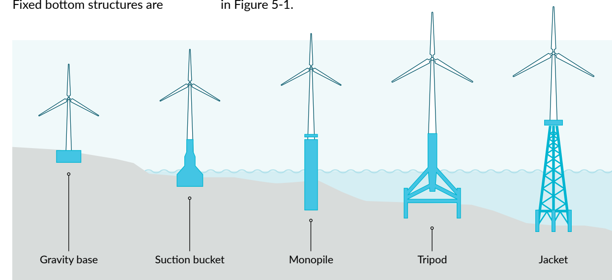
Figure 5-1 Different types of fixed-bottom offshore wind foundations [35]
