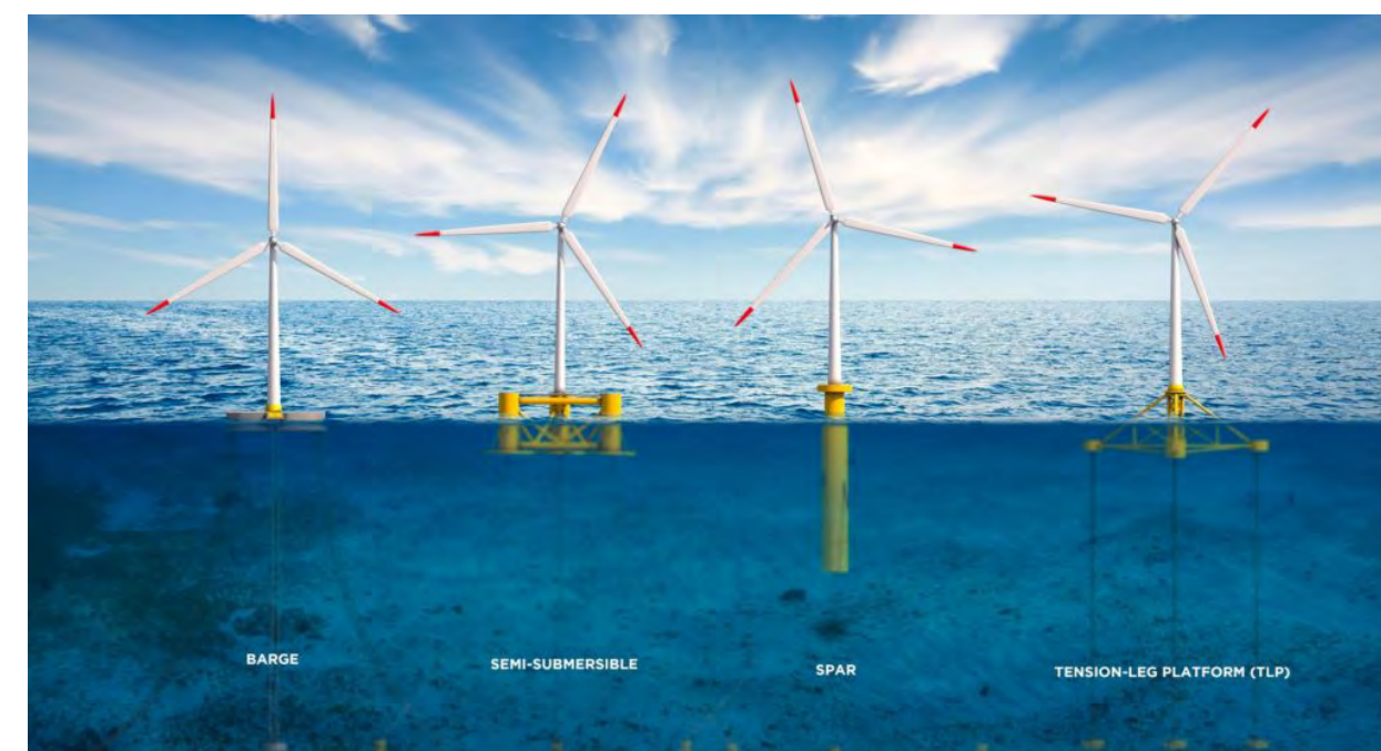
Figure 5-2 Different types of floating offshore wind foundations [36]
